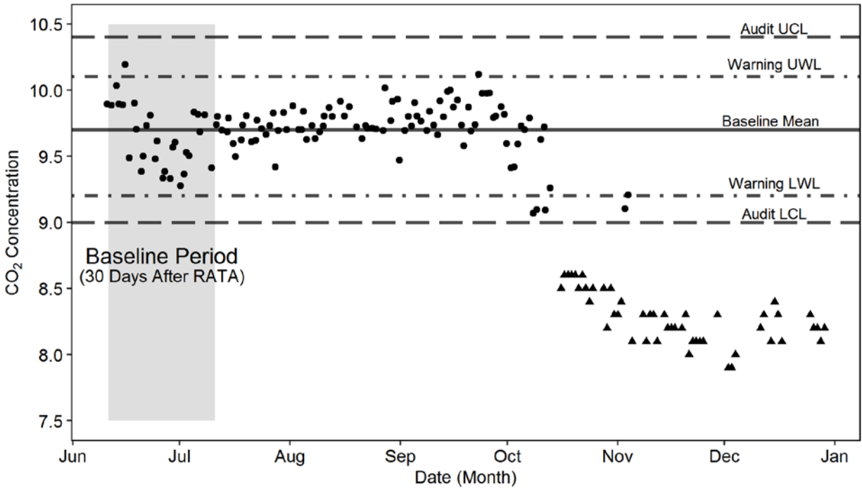
Figure 4. Typical CO 2 control chart
