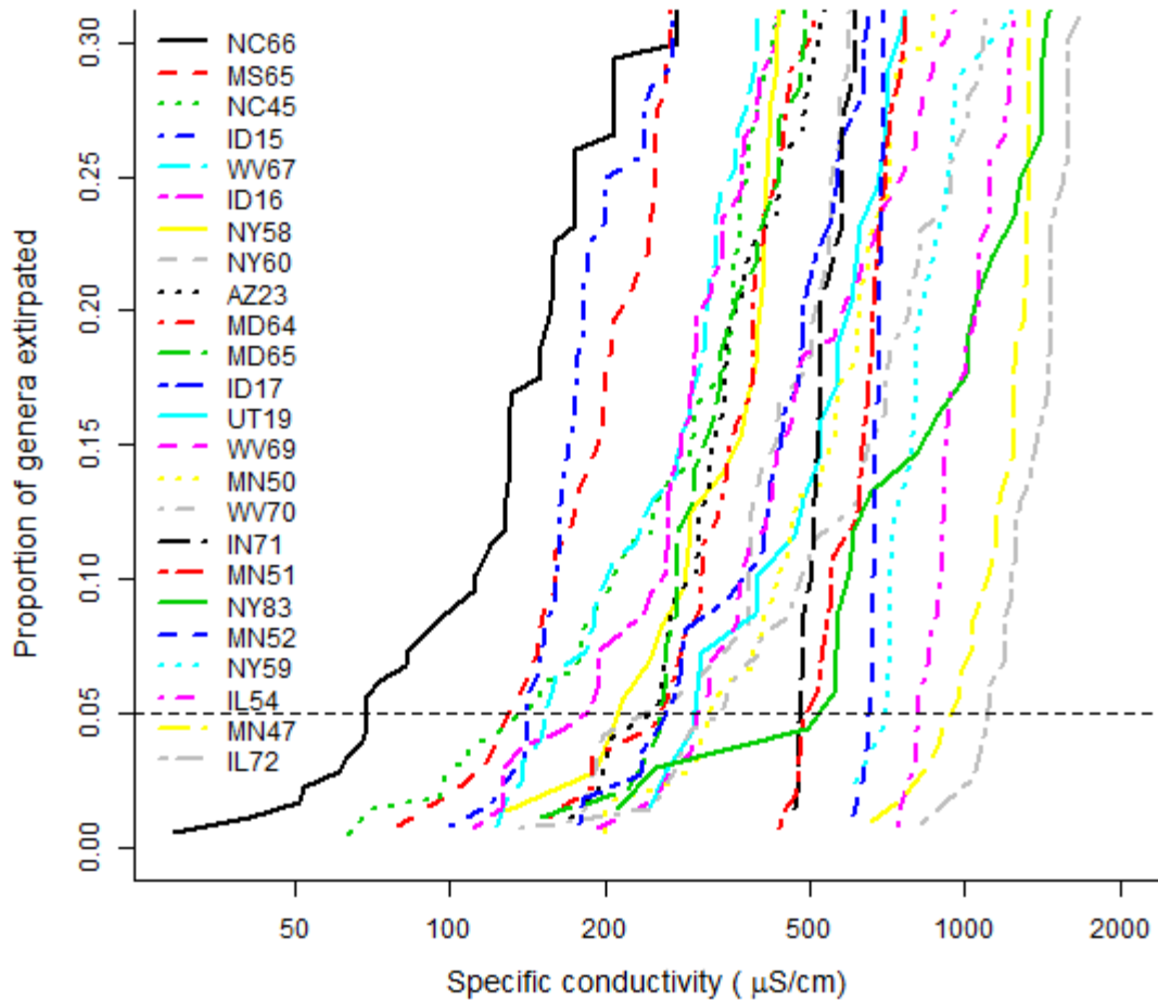
Figure D-3. The lower 30% of the 24 extirpation concentration distributions (XCDs). Hazardous concentration ( HC_{05} ) is the specific conductivity (SC) at the 5 th centile of each XCD (horizontal dashed line). The ecoregion legend and XCDs are ordered from lowest (NC66) to highest (IL72) HC_{05} and roughly from lowest to highest background SC. Untransformed SC values shown on log 10 scaled x -axis.
