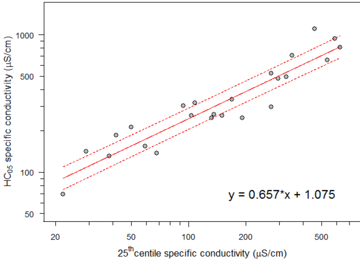
Figure D-4. Benchmark-to-criterion empirical model. The x-axis shows the untransformed background specific conductivity (SC) estimated at the 25 th centile for 24 state data sets, scale is log10. Also scaled (log10), the y-axis shows the untransformed 5 th centile hazardous concentrations (HC 05 ) of extirpation concentration distributions (XCD) shown in Figure D-3. Solid line is the log10-log10 linear regression line. Dotted lines demarcate the 50% prediction intervals (PI). That is, the probability that any new HC 05 would plot within those bounds is 50% and only 25% are expected to fall below the lower prediction limit (PL). Pearson’s correlation coefficient ( r = 0.93 ). Data in Table D-2.
